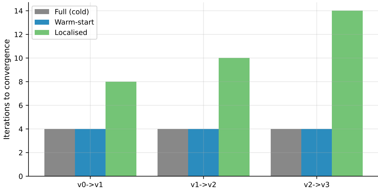
Group C - Iterations per update strategy
